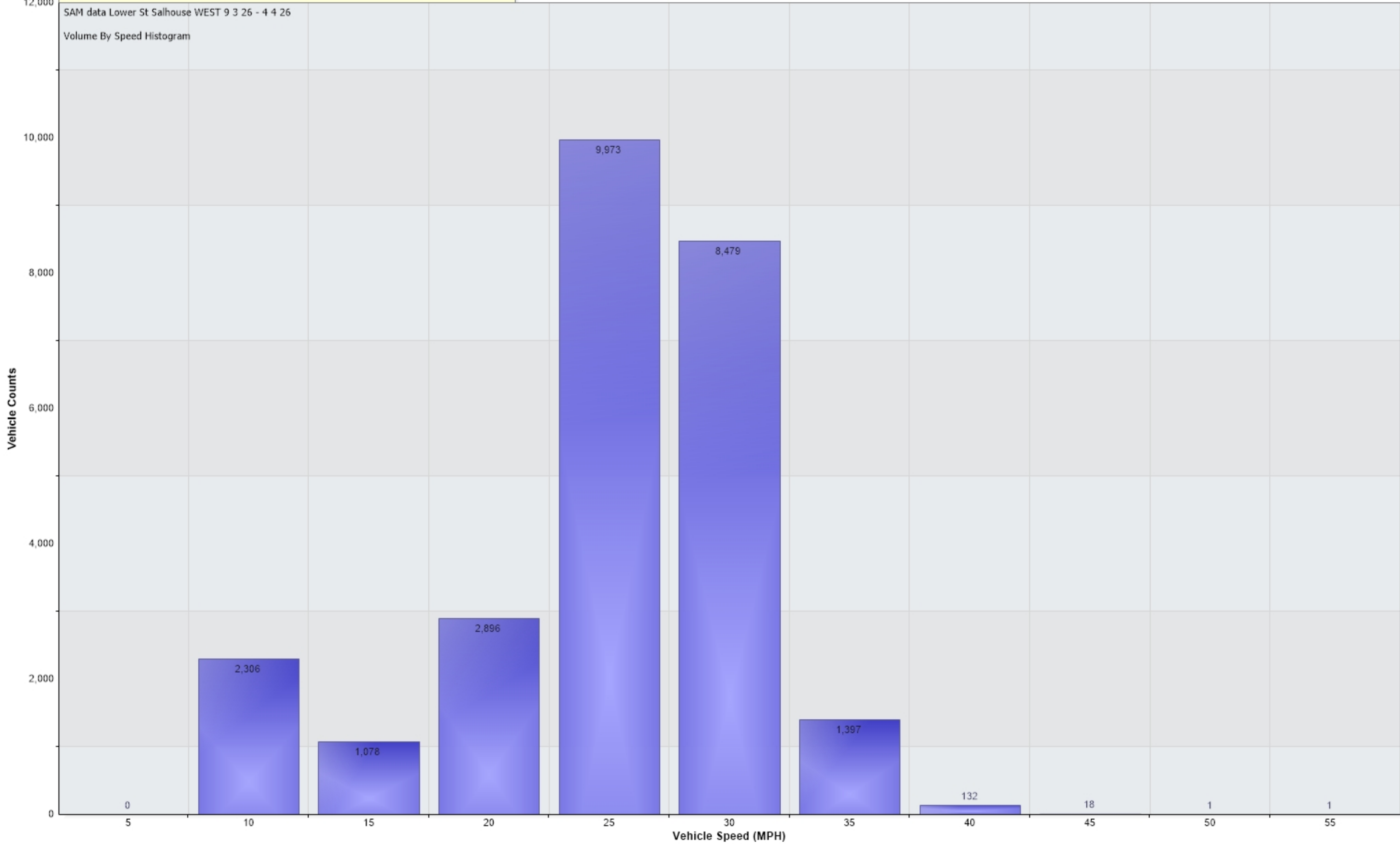
Vehicle Counts Vs. Speed [SAM data Lower St Salhouse WEST 9 3 26 - 4 4 26: Incoming]
